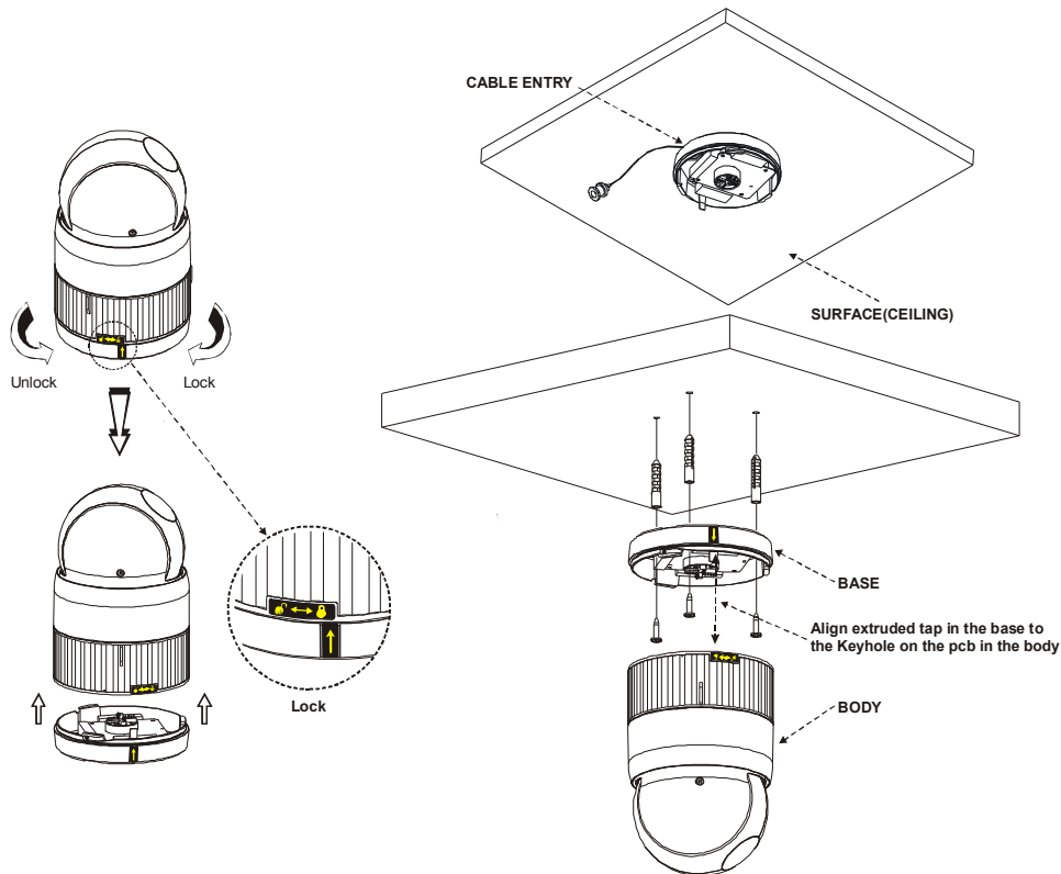
Figure 3 – Installation
