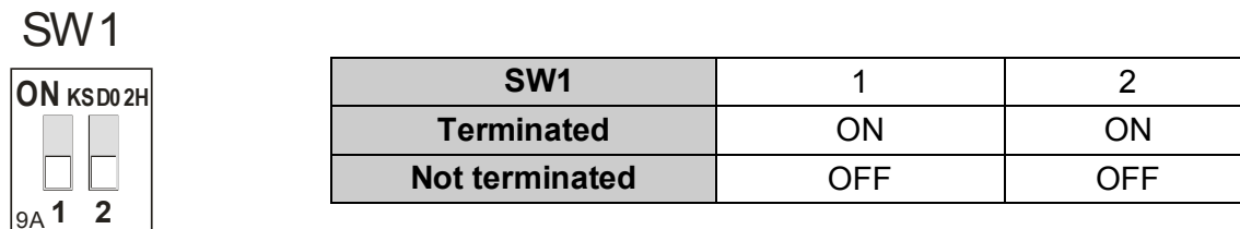
Figure 6 – Setting Dome Camera Termination
