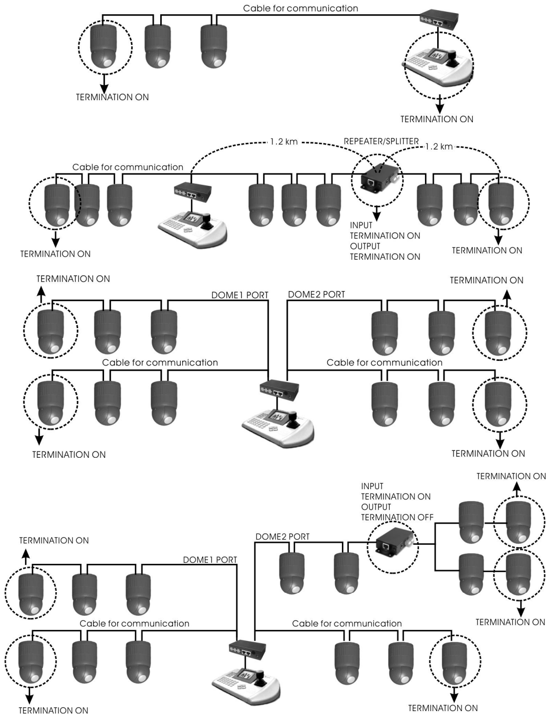
Figure 7- Termination Diagram
