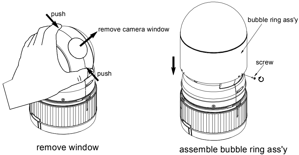
Figure 2 – Assemble bubble ring ass'y
