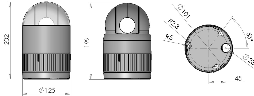
Figure 10 – Dimension
